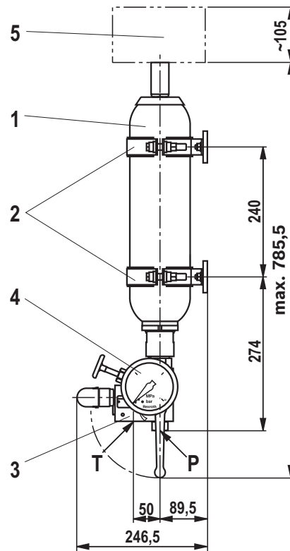
Bladder-type accumulator 2.5 liter
