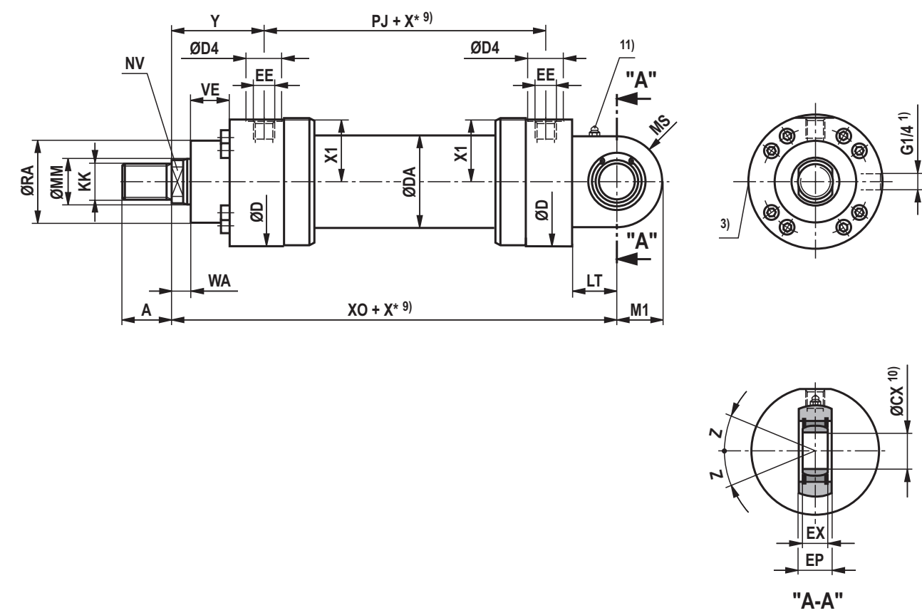
CDH1 MP5: With seal design "A", "B" and AL Ø 160 to 320 mm
