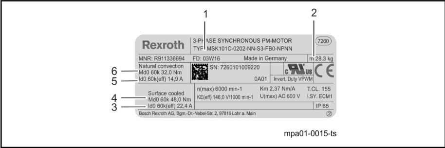
Fig. 5-7: Identification MSK
