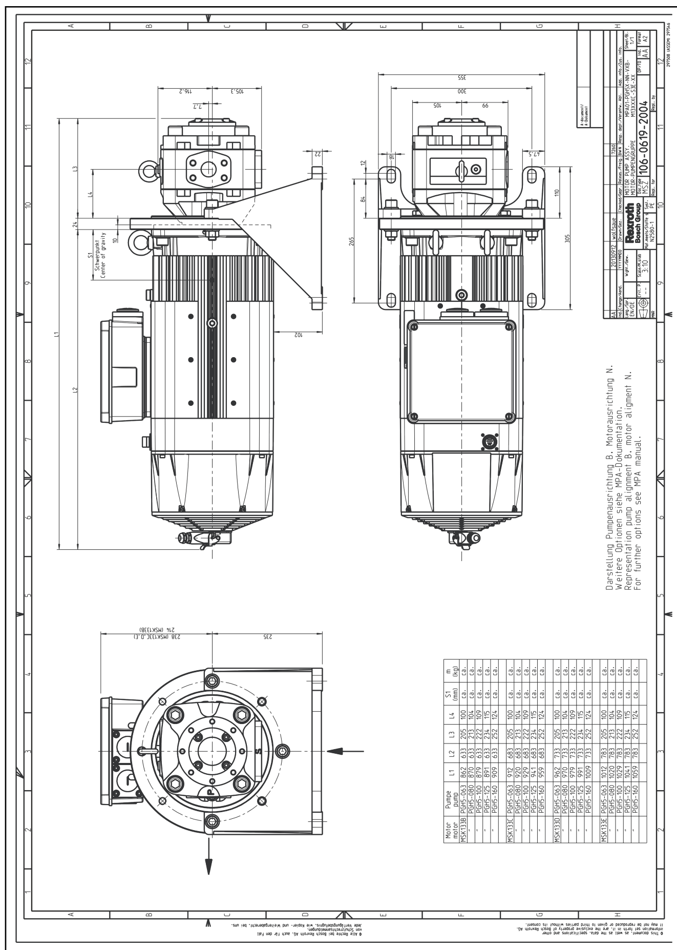
Fig. 17-23: MPA01-PGH5x-NN-VxN-M13xxxC-S3E-NN(flange fastening)
