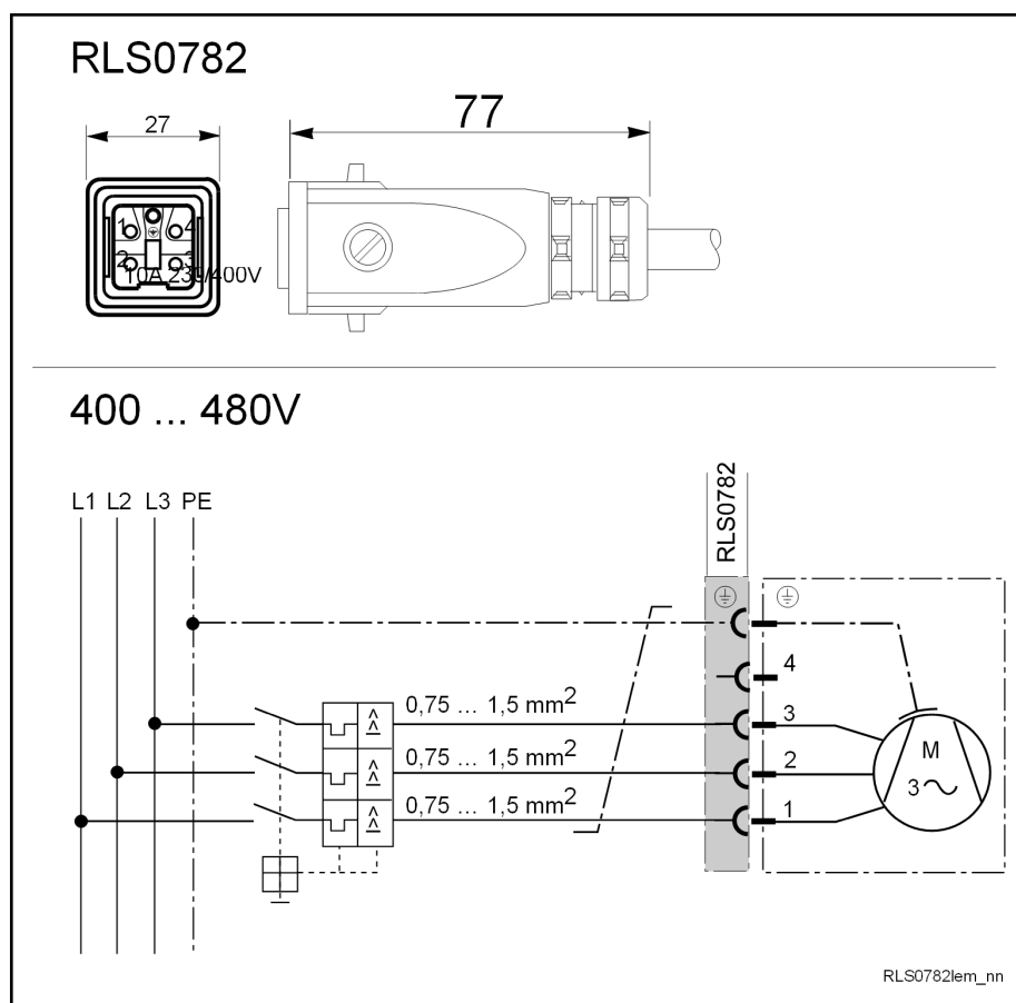
Fig. 8-8: Fan connection 3-phase with protection switch
