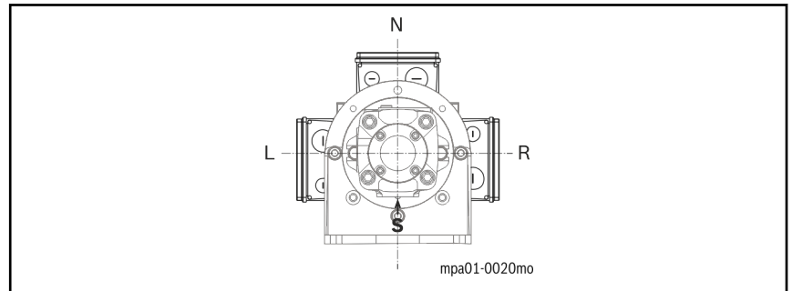
Fig. 7-7: Motor assembly direction
