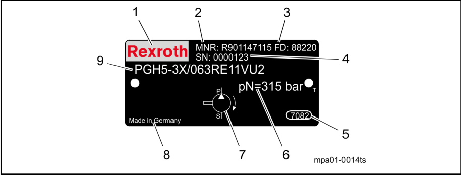
Fig. 5-6: Type plate internal gear pump
