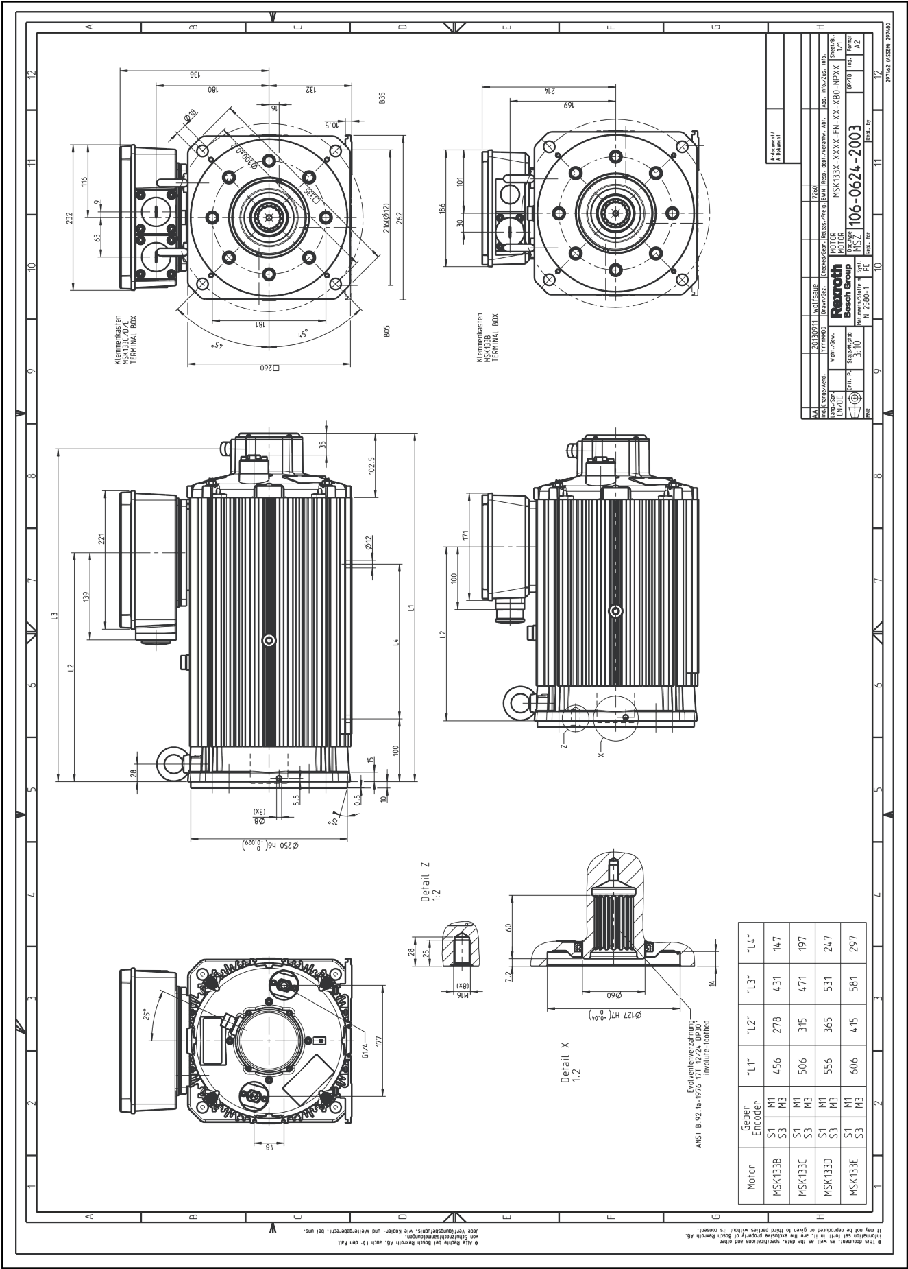
Fig.17-24: MSK133 - -FN
