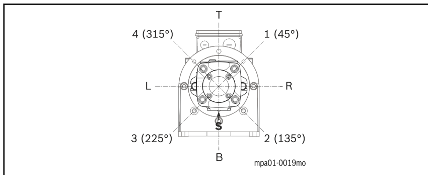
Fig. 7-3: Pump assembly mounting direction
