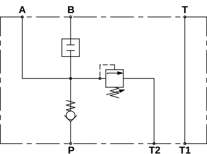
Manifold Hydraulic Diagram
