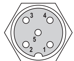
Top view mating connector
