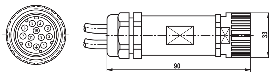
Allocation of connector or mating connector and cable set
