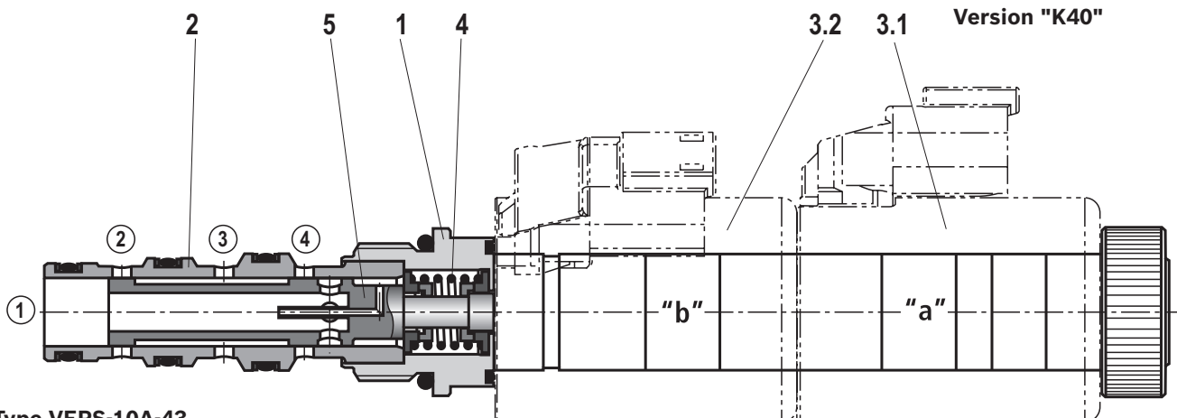
Type VEPS-10A-43...
